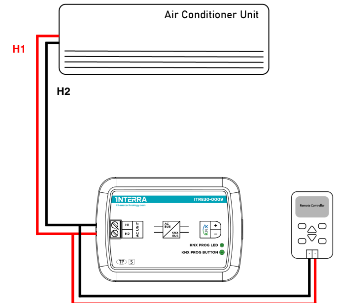
Gree AC - KNX Gateway — Single Indoor Unit + Remote Controller :
