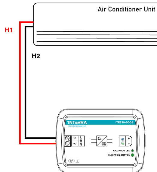
Gree AC - KNX Gateway — Single Indoor Unit :
